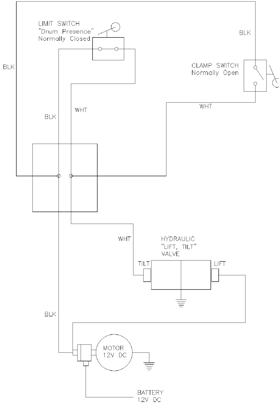
ELECTRICAL SCHEMATIC MORSTAK
