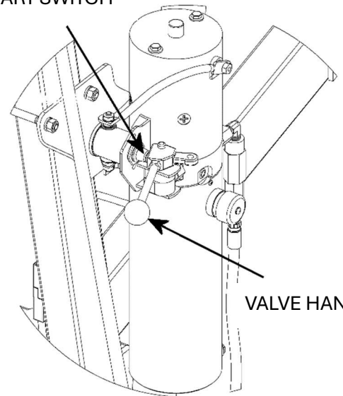
START SWITCH
